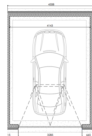
SINGLE GARAGE
